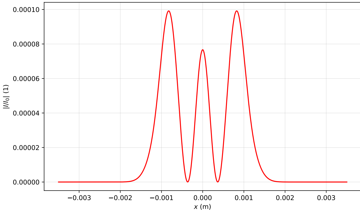
Intensity profile I(x, y = 0, z = 0.557)/I_0 , P_{in}=1.0P_{cr} , artificial time
